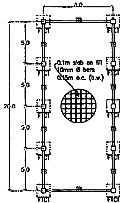
FOUNDATION PLAN
