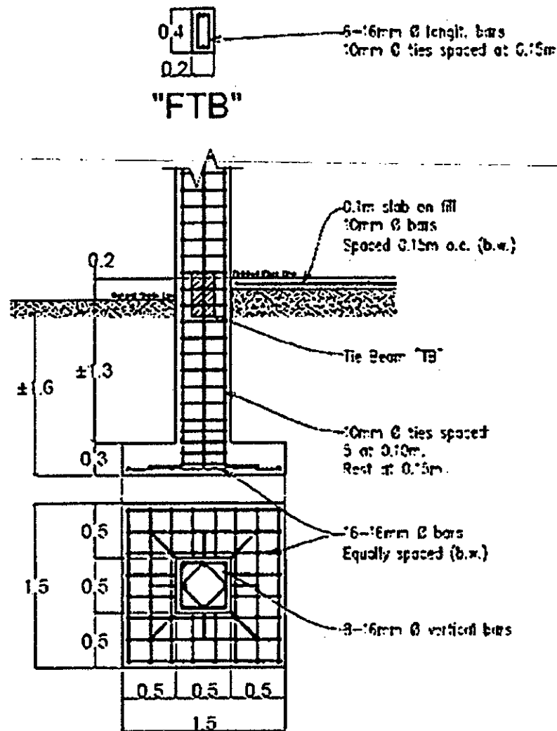
SECTION DETAIL COLUMNS AND BEAMS
