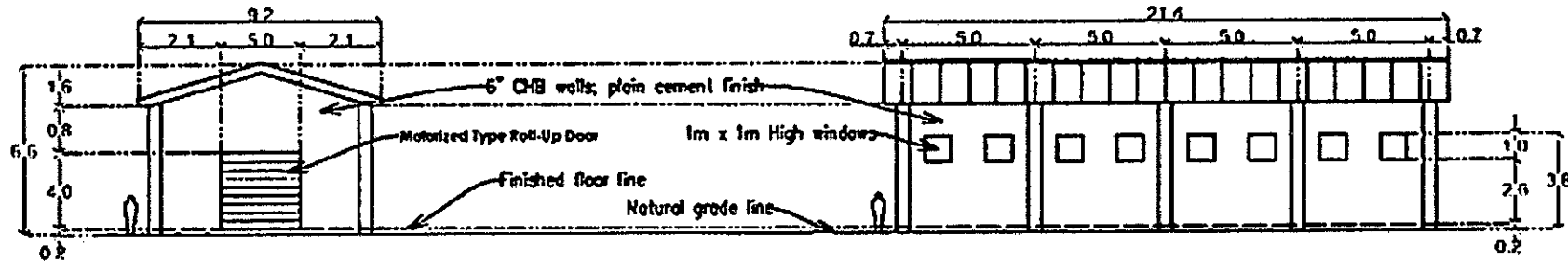
FRONT ELEVATION
