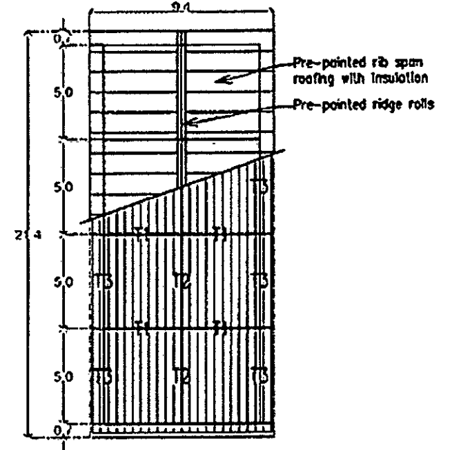
ROOF PLAN
